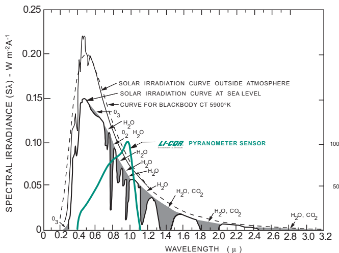
Figure 1. The LI-200SA Pyranometer spectral response is illustrated along with the energy distribution in the solar spectrum (3).
